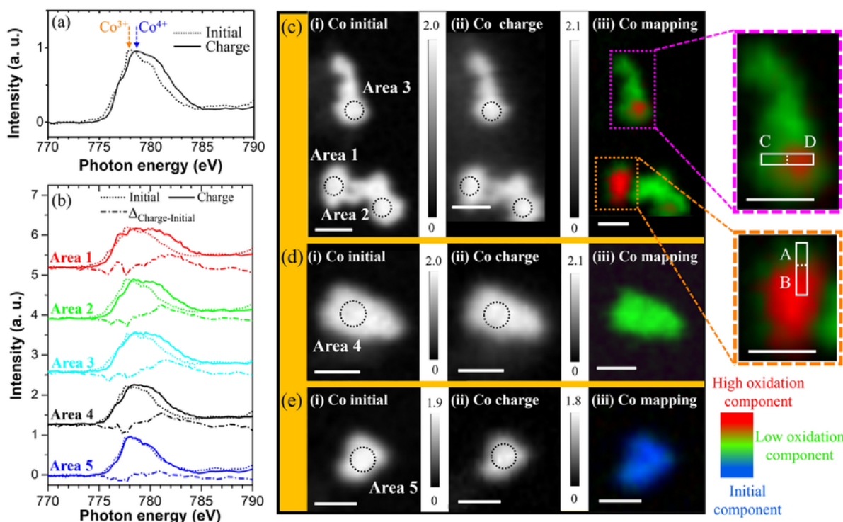
An example of STXM characterization of LiCoO 2 particles used as cathode material in lithium-ion batteries, in their initial state and after charging (lithium intercalation), showing redox reaction occurring for Co atoms
