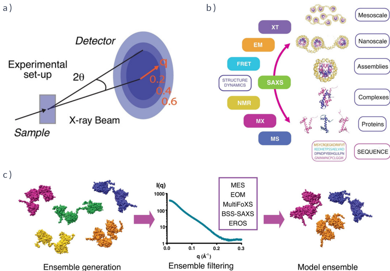
(a) A scheme of a typical SAXS experiment, (b) functional potential of the SAXS technique, compared to other structural biology methods. (c) SAXS-based ensemble modelling
