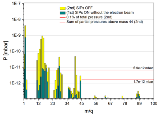
Figure 3: RGA of one vacuum sector without electron beam and with SIPs switched on and off.
