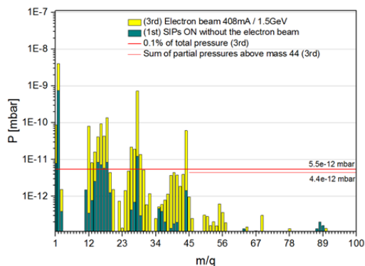
Figure 4: RGA with and without electron beam.
