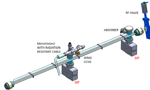
Figure 2: Vacuum chamber of the straight section.
