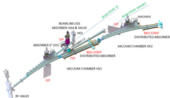
Figure 1: Vacuum chamber of the arc section.
