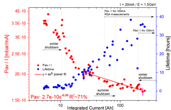
Figure 5: The evolution of P_{av}/I and lifetime versus integrated current.
